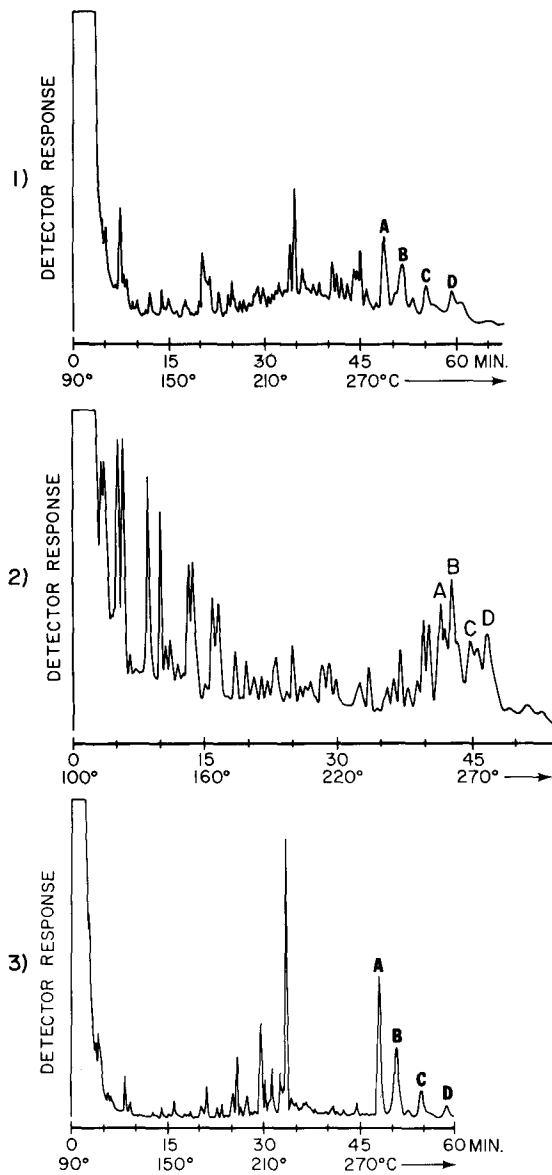
Figure 1. The gas chromatograms of the BSA-treated methanol eluate of the Christiaensen Basin mud (1), the P-21 sample (2), and the Ward' Island sewage sludge (3). A 6'x1/8" o.d. glass column packed with 3% OV-1 on chromosorb W(HP) was used in (1) and (3). A 6'x1/4" glass column packed with the same material was used in (2).
