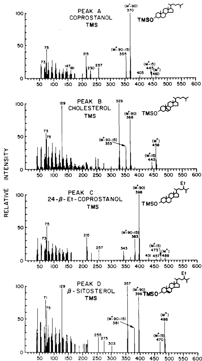
Figure 2. The mass spectra of the TMS derivatives of coprostanol, cholesterol, 24β-ethyl coprostanol, and β-sitosterol in the Christiaensen Basin mud sample.
